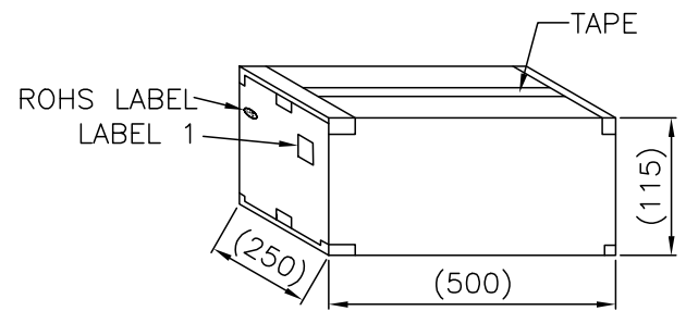
PACKING
