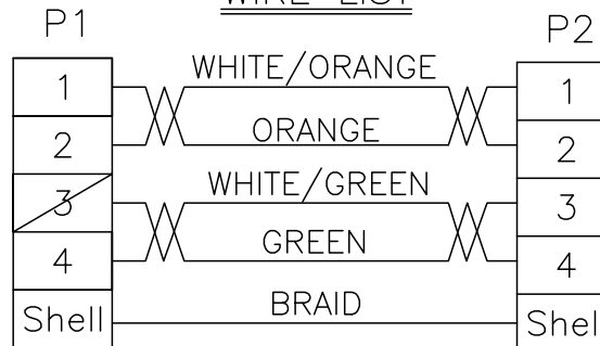
WIRE LIST
